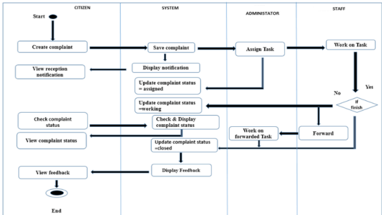
Figure 4.4: Activity Diagram
