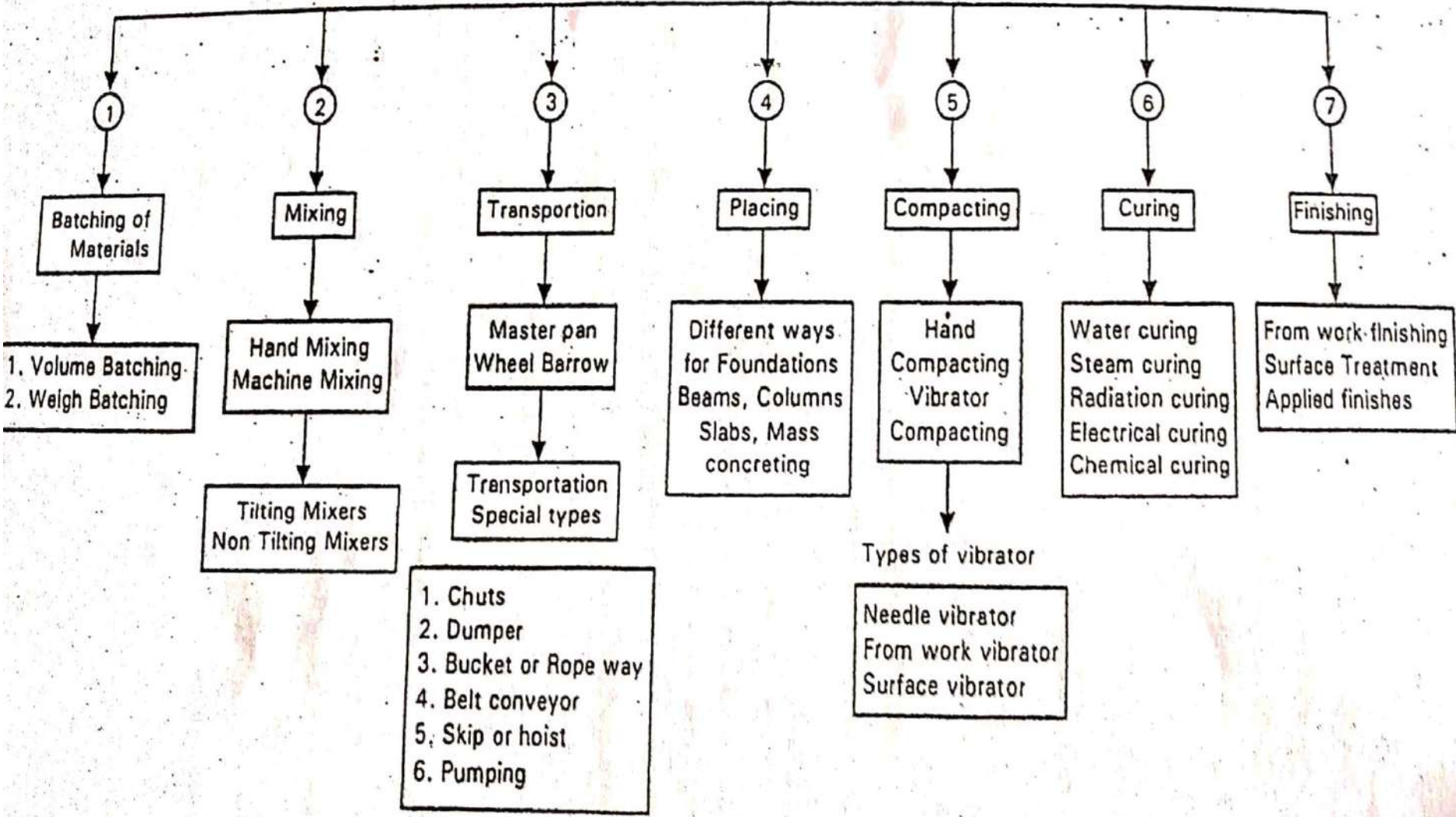
Fig. 2.9 : Flow chart for production of concrete
